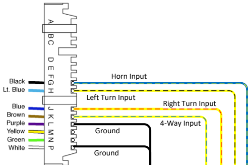
GM Steering Column Connector
